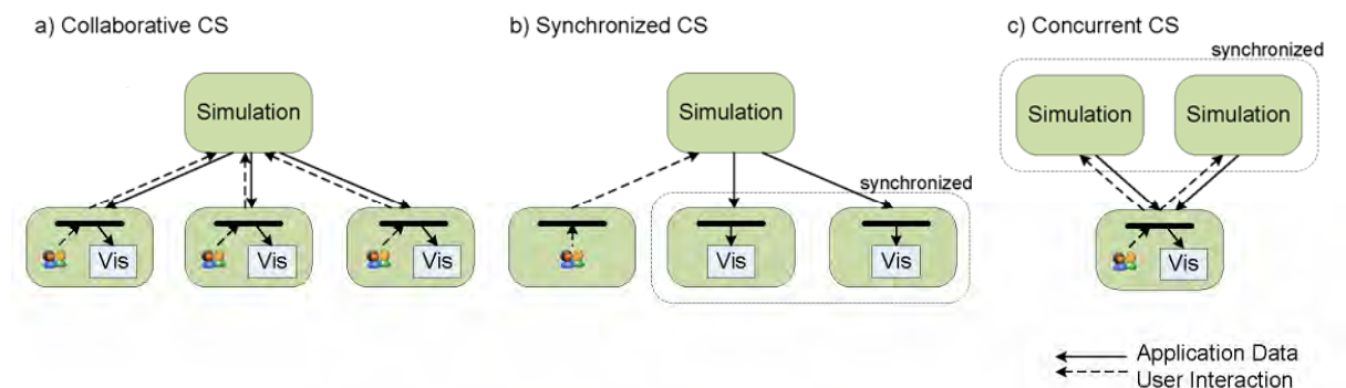
Figure 2 Three additional use cases of computational steering of distributed virtual reality systems
