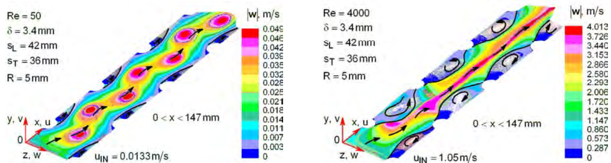
Figure 3: Velocity field in the plane y = 0 at Re = 50 and Re = 4000 .
