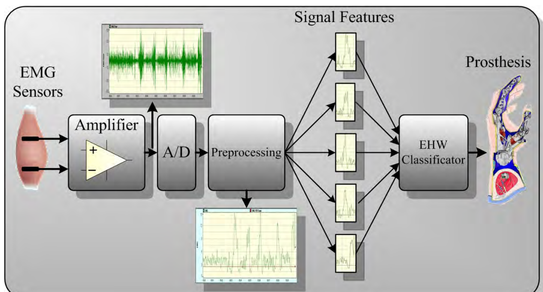
Figure 2 Architecture of muscle signal classifier
