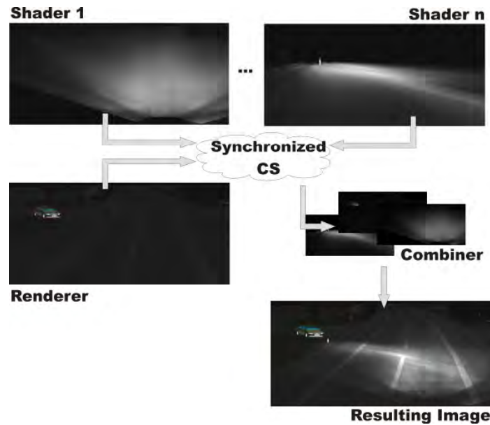
Figure 5 Composing synchronously rendered frames
