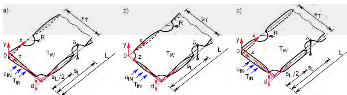
Figure 2: Geometry and dimensions of the three-dimensional simulated domains.
