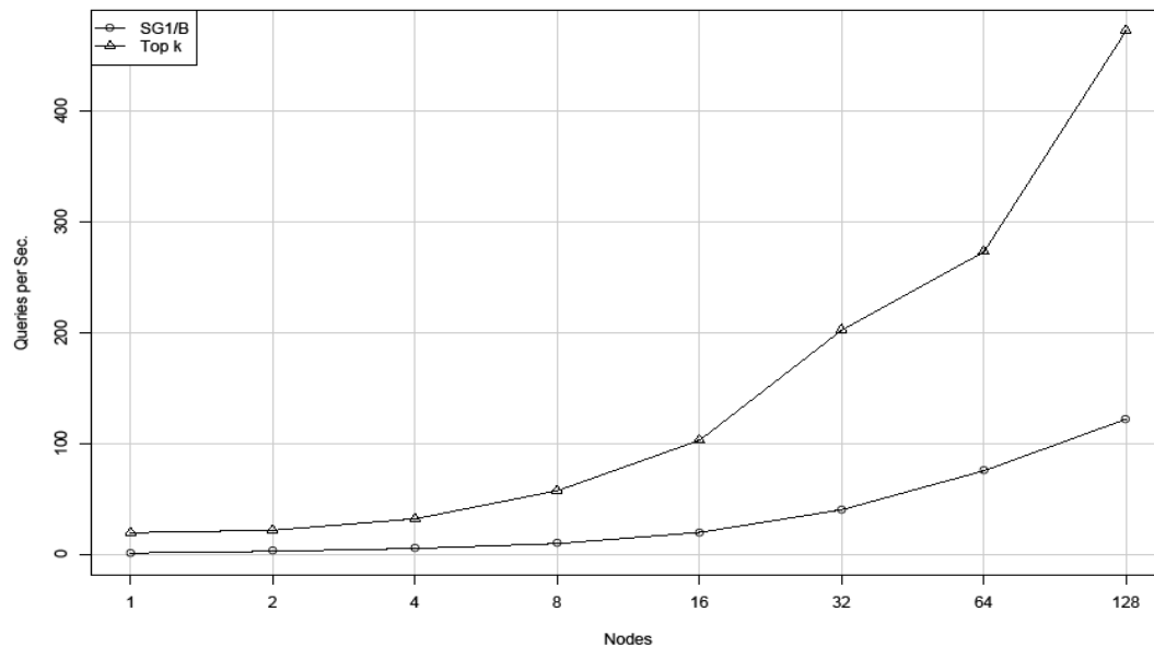
Figure 2: Evaluation of top k queries (on Arminius)
