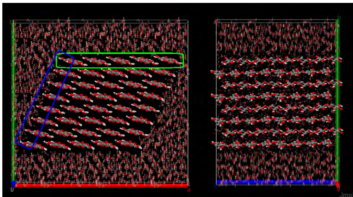
Figure 2: Simulation-box with 40 cellulose chains (8 layers with 5 chains each). Each chain consists of 8 glucose rings. The box is filled with a total of 3269 water molecules (transparent) and is shown as a projection of the X-Y-plane (left side), and the Y-Z-plane (right side). The chains are oriented parallel to the Z-axis (blue), while the rings are laying in the X-Z-plane (not shown). The resulting theoretical cellulose crystal represents a polar (blue border) and a non polar surface (green border).
