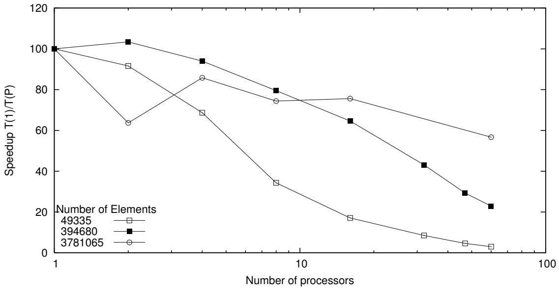
Figure 10: Speedup for the resolvent step.
