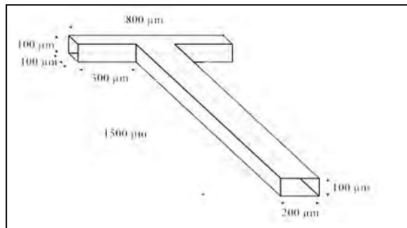
Figure 1 Mixing zone of the T1-micro-reactor - investigated by 3D simulations.
