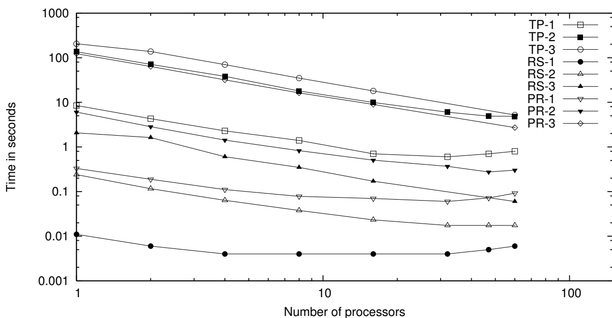
Figure 12: Simulation time for a complete time step.
