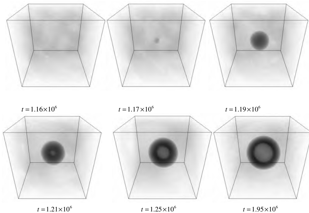
Figure 1: Aggregation morphology of amphiphilic diblock copolymers in dilute solution in 3D at various times. Only the density distribution of A is shown. The Flory-Huggins parameters are \chi_{BS} = -0.45 , \chi_{AS} = 1.2 , \chi_{AB} = 1.05 ,
