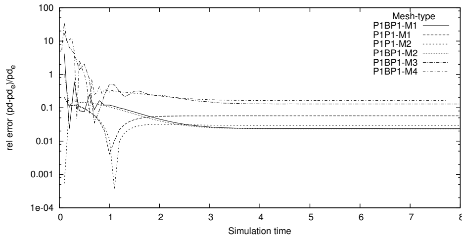
Figure 5: Relative error of the pressure difference.
