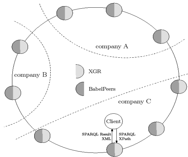
Figure 3: Running BabelPeers and XGR
