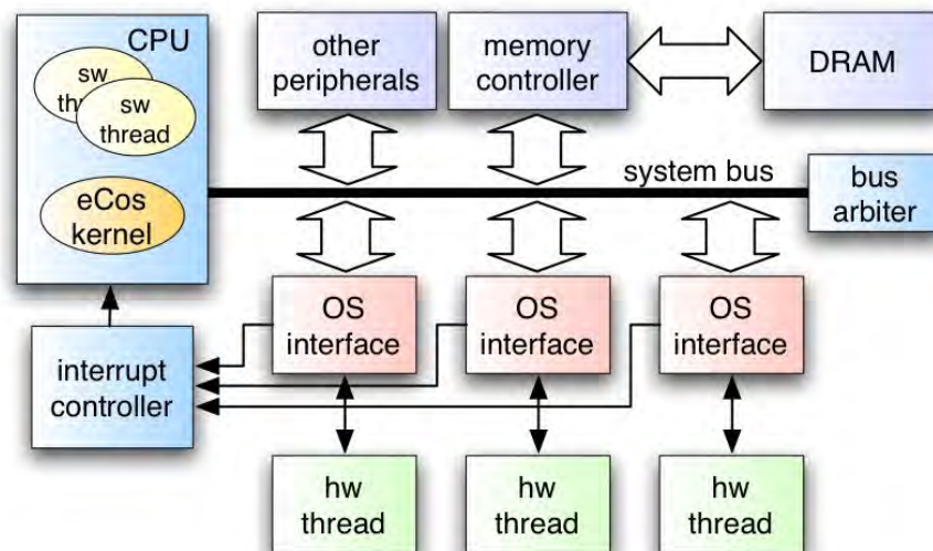
Figure 4. ReconOS run-time system architecture
