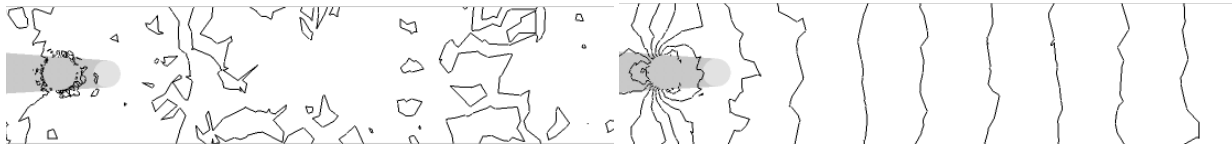
Figure 2: Iso-lines of the P1/P1 and P1-Bubble/P1 approach
