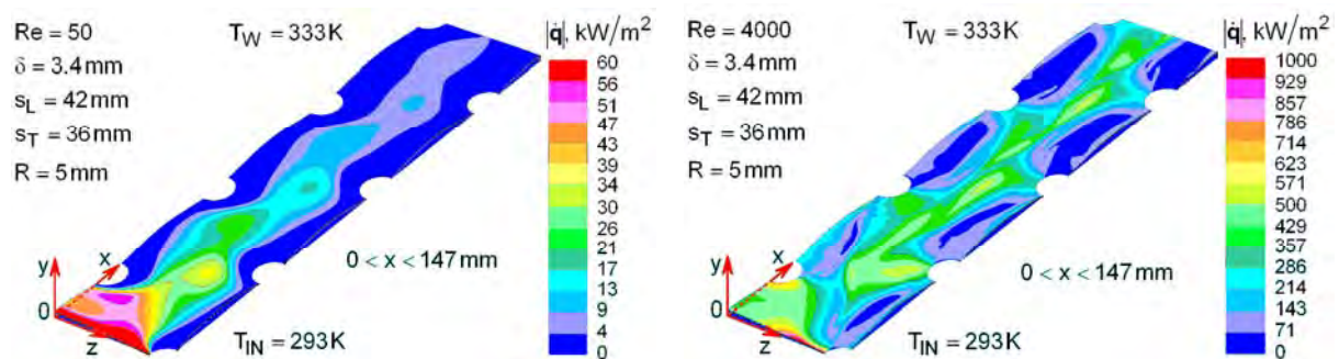
Figure 4: Wall heat flux field at Re = 50 and Re = 4000 .
