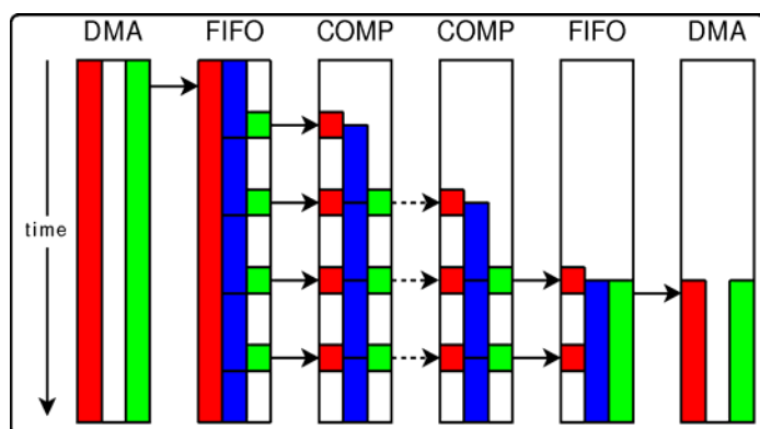
Figure 2: Task graph of an algorithm mapped to a pipelined architecture in an FPGA
