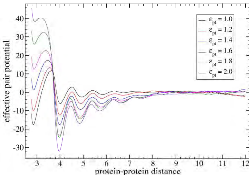
Illustration 3: Effective pair potential between two proteins in the fluid phase
