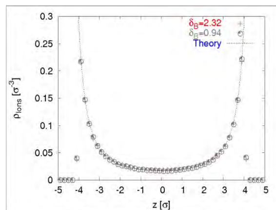
Illustration 2: Counterion distribution in a channel with charged walls for different slip lengths in comparison to Poisson-Boltzmann-theory.
