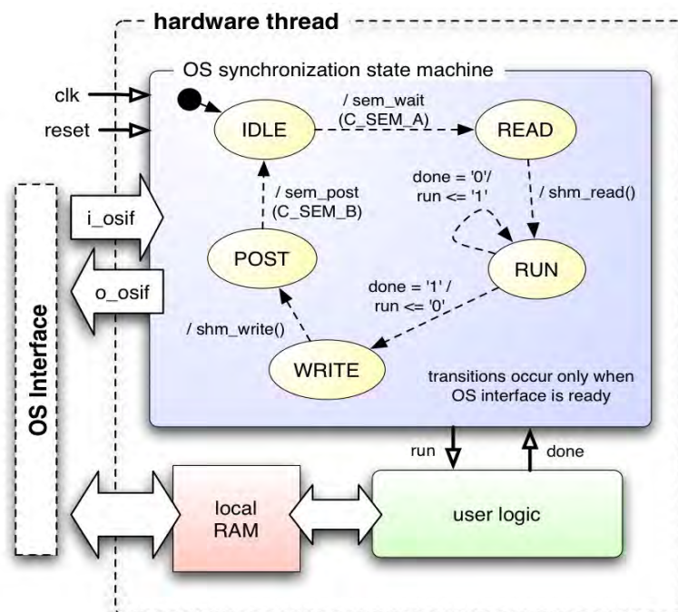
Figure 3. Hardware thread structure
