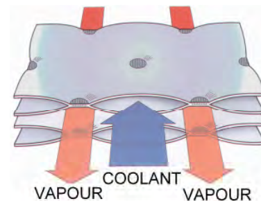
Figure 1: Fluid flow arrangement in thermoplates (DEG-Engineering).
