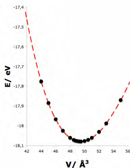
Figure 2: Calculated Energy versus Volume Curve (Points) and a fit to the 3 rd order Birch-Murnaghan equation of state (Curve).
