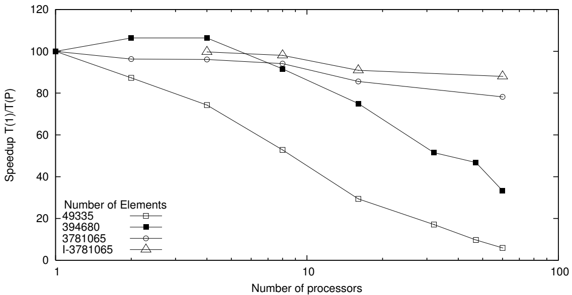
Figure 11: Speedup for the pressure correction.
