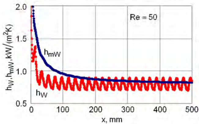
Figure 5: Distribution of the heat transfer coefficient
