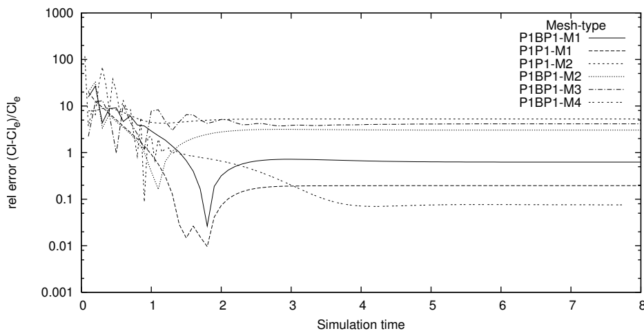
Figure 4: Relative error of the lift coefficient.
