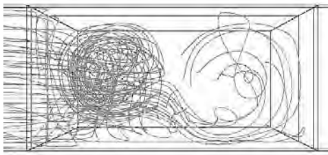
Figure 2 Flow trajectories crossing the symmetry plane in engulfment flow. View into the mixing-channel.
