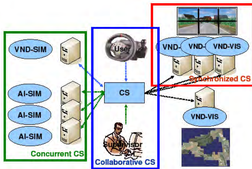
Figure 4: Extended use cases in the Virtual Night Drive application
