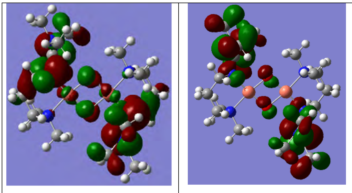
Figure 4: left: HOMO with 70% guanidine contribution, right: HOMO-2 with 70% guanidine contribution
