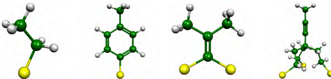
Figure 2: Thiolates used in our pulling simulations. From left to the right: an alkylic thiolate, an aromatic thiolate, a bidentate thiolate and a tridentate thiolate.
