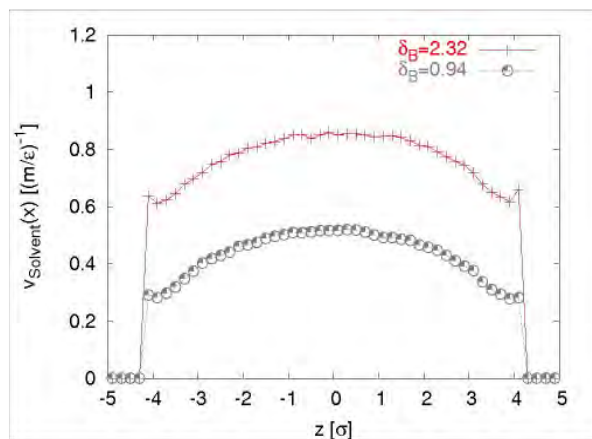
Illustration 1: Counterion-induced electroosmotic flow of the solvent for different slip lengths.
