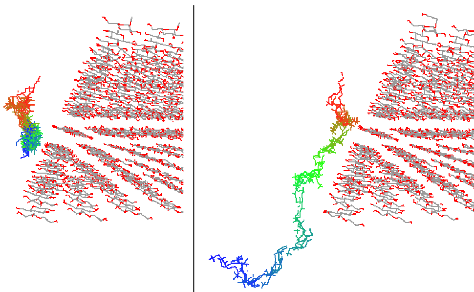
Figure 3: Trajectories of ligand movement of amide 2.1 (left) and amine 1.1 (right) at the polar cellulose surface. The Figure depicts the ligand positions in time-steps of 5 ps with a time resolved spectral color code from red ( t=0 ps) towards blue ( t=250 ps) with a constant picture of the cellulose at t=0 ps.
