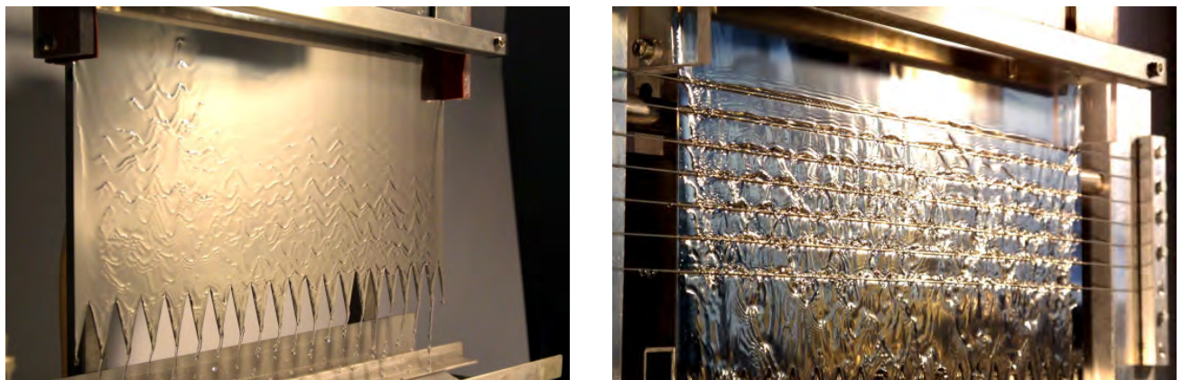
Figure 1: Wavy falling water film without (top) and with (bottom) turbulence wires
