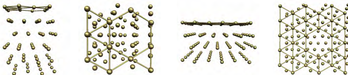
Figure 1: Two views of the six-layer gold slab (on the left) and two views of the four-layer slab (on the right)
