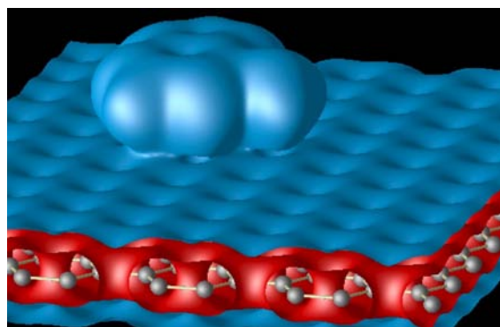
Figure 1: Isosurfaces of the calculated total valence charge density of adenine adsorbed on graphite (0001). The positions of the carbon atoms in the uppermost graphene sheet are indicated. From Ref. [1].
