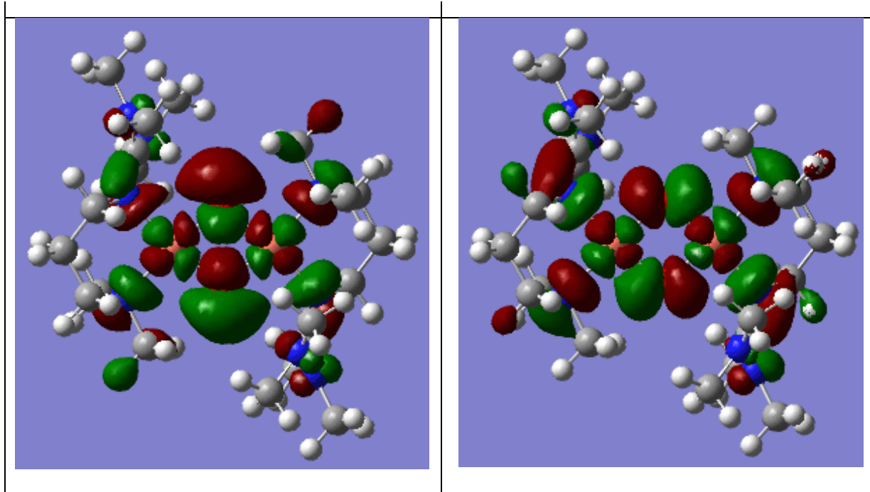
Figure 5: left: LUMO with 34 % Cu and 44 % O contribution, right: LUMO+1 with 37 % Cu and 34 % O contribution
