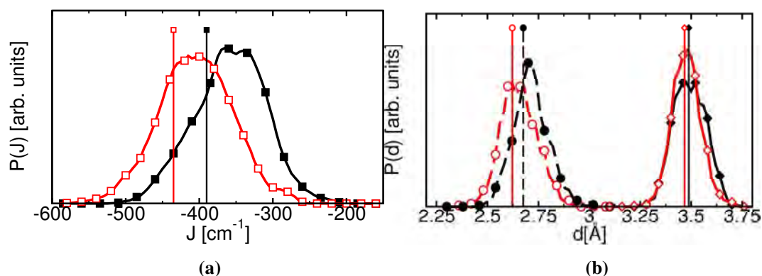
Figure 3: Probability distribution functions of (a) the Fe-Fe (broken line, circles) and S1-S2 distance (solid line, diamonds) and (b) of the coupling constant J (solid line, squares) obtained from AIMD of the [\text{Fe}_2\text{S}_2(\text{SH})_4]^{2-} cluster in vacuo using the BS (black, filled symbols) and EBS (red, open symbols) schemes. The corresponding values obtained for the minimum energy structures are shown as vertical bars with a symbol.
