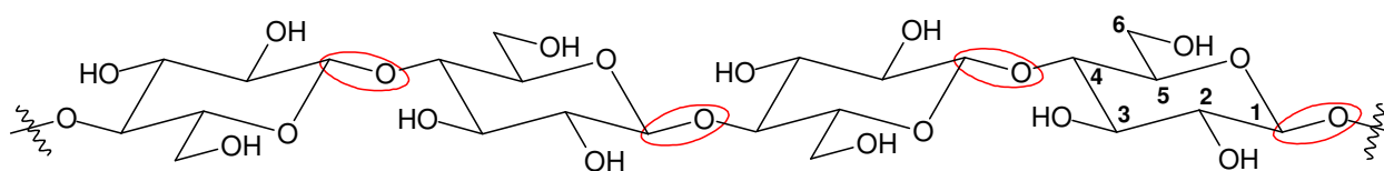
Figure 1 Chemical structure of a single cellulose strand made from four single glucose units covalently connected by \beta -1,4-glycosidic linkages (red circles)
