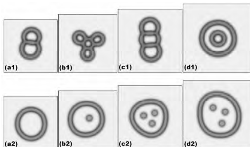
Figure 2: Manifold vesicles at the various initial number density of stable nucleus c_{ini} and Interaction parameters \chi_{BS} , Black and grey stand for solventphilic and solvent-phobic regions. \chi_{BS} = -0.3 (top group), \chi_{BS} = -0.6 (bottom group): c_{ini} = 9.0 \times 10^{-4} R_g^{-2} (a1, a2); c_{ini} = 7.44 \times 10^{-4} R_g^{-2} (b1,b2); c_{ini} = 6.25 \times 10^{-4} R_g^{-2} (c1 and c2); c_{ini} = 5.33 \times 10^{-4} R_g^{-2} (d1,d2). Black and grey as in Figure 1
