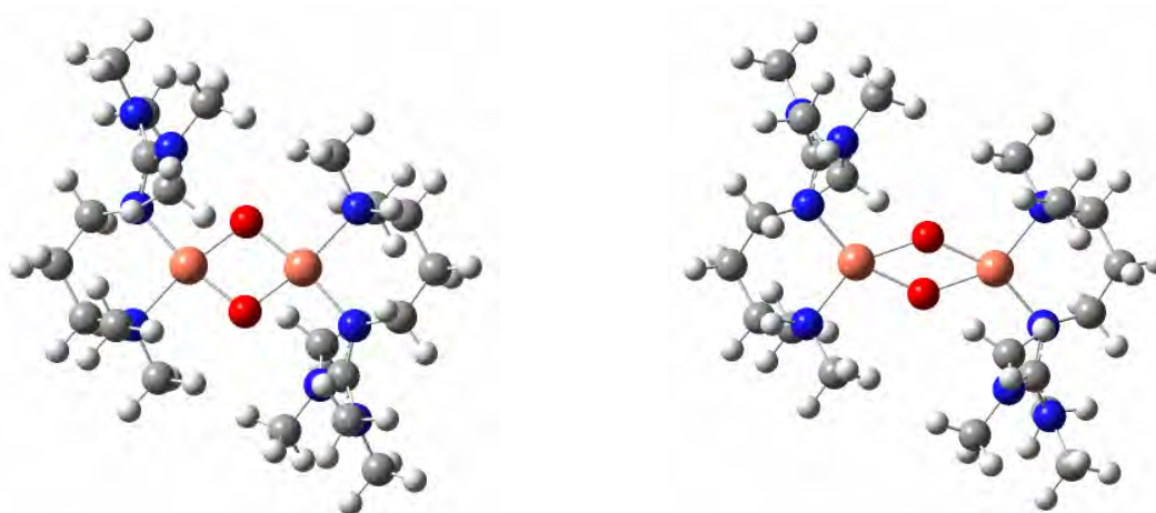
[(\text{TMGdmap})_2\text{Cu}(\text{III})_2(\mu\text{-O})_2]^{2+} ( O species)
