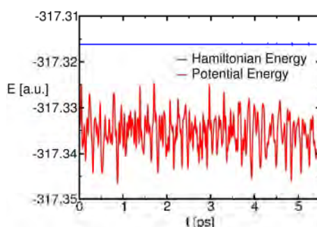
Figure 1: The conserved Hamiltonian energy (blue) on the scale of the potential energy (red). All energy values are reported in a. u.
