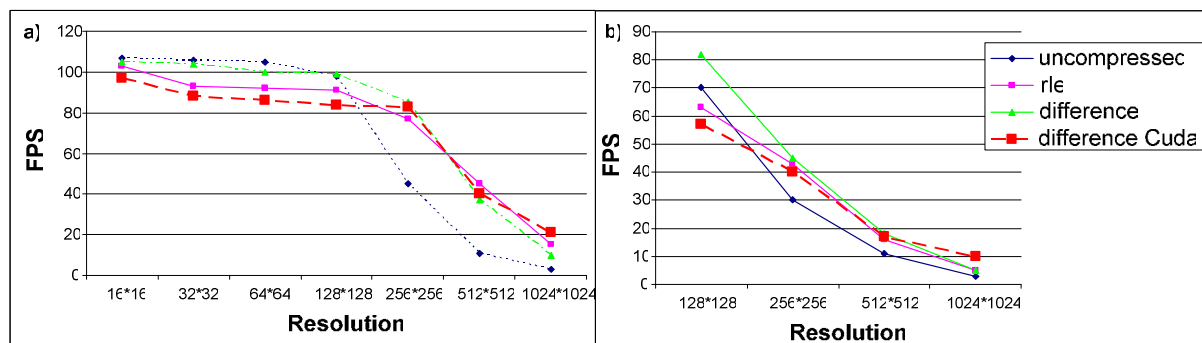
Figure 3: Benchmarking results with A) Teapot and B) Virtual Night Drive
