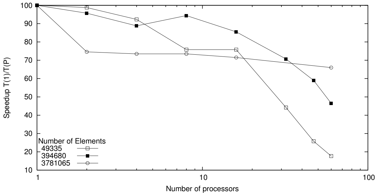
Figure 9: Speedup for the transport step.
