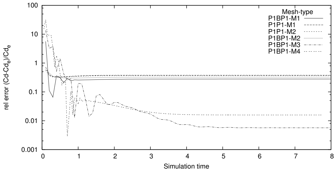
Figure 3: Relative error of the drag coefficient.
