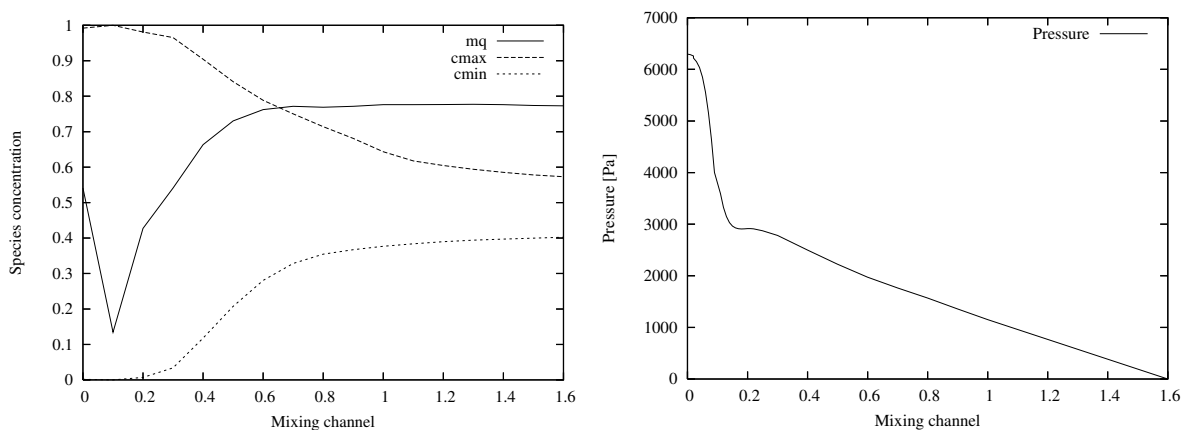
Figure 6: Pressure and Species distribution along the outflow channel.
