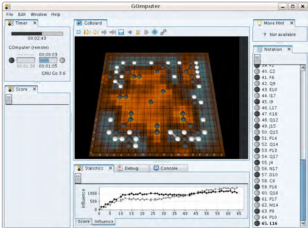
Figure 1: The graphical user interface visualizing the influence feature
