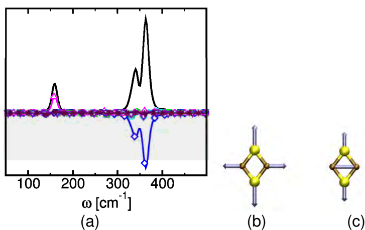
Figure 4: Power spectrum of J (black curve) together with the frequency dependent correlation between J and the individual vibrational components of the \text{Fe}_2\text{S}_2 core dynamics obtained from the EBS-AIMD of the cluster in vacuo; A_{g,A} (magenta), A_{g,D} (blue), other colors are the rest of the modes. Ideal symmetry adapted modes (b) A_{g,D} and (c) A_{g,A} . Yellow spheres are sulfur atoms and grey spheres are iron atoms.
