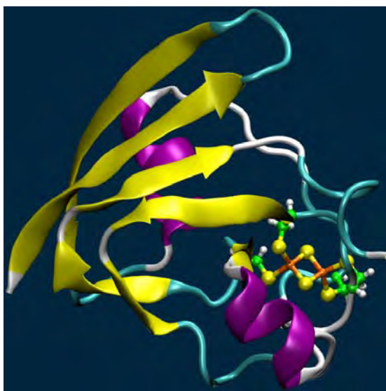
Figure 5: Anabaena ferredoxin; ball and sticks are used to show the quantum part of the system used in the QM/MM calculations. Color code: carbon (green), yellow (sulfur), white (hydrogen), orange (iron)
