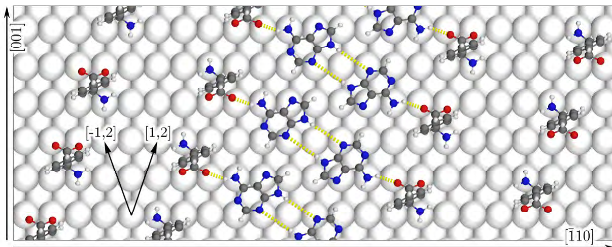
Figure 3: Molecular model derived in Ref. 2 for phenylglycine co-adsorbed with adenine forming dimer rows along the [1,2] direction on Cu(110). Hydrogen bonds are indicated with yellow lines.
