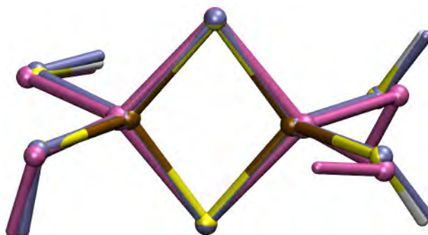
Figure 2: [\text{Fe}_2\text{S}_2(\text{SH})_4]^{2-} structures obtained by structure optimizations in vacuo in different spin states. The structure corresponding to the BS state is ice-blue, the HS structure is mauve and for the EBS structure the iron, sulfur and hydrogen atoms are shown in brown, yellow and white, respectively.
