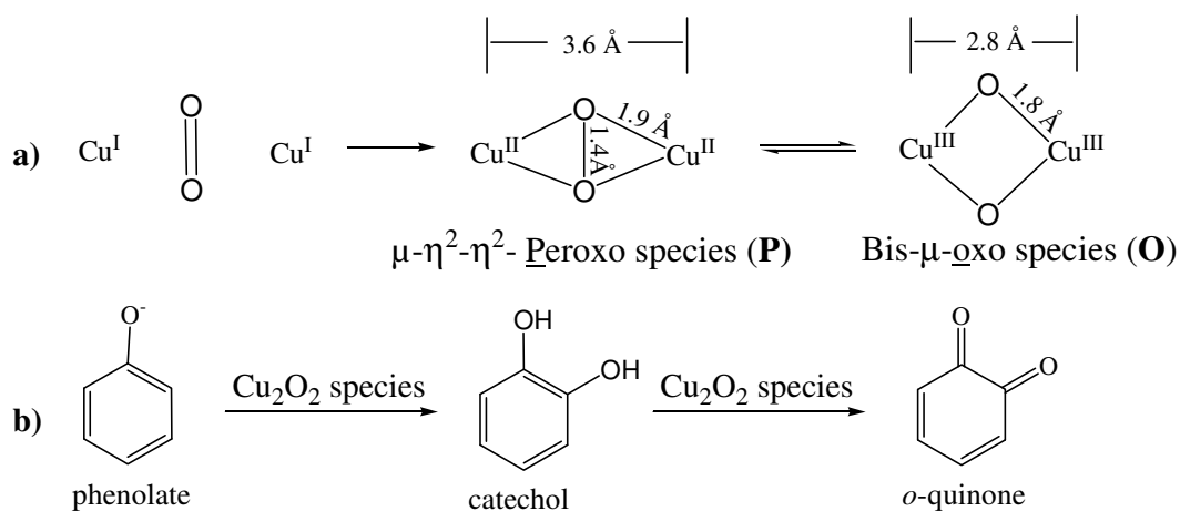
Scheme 1: a) Oxygen activation by copper complexes, b) Hydroxylation of phenolates and oxidation of catechols
